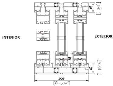
CROSS SECTION FOR 3 PANEL (Vertical Section)
